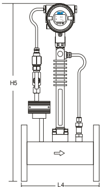
Flange Type with T/P Sensor
