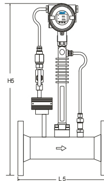
Reduced Bore Type
