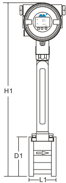
Wafer Type
